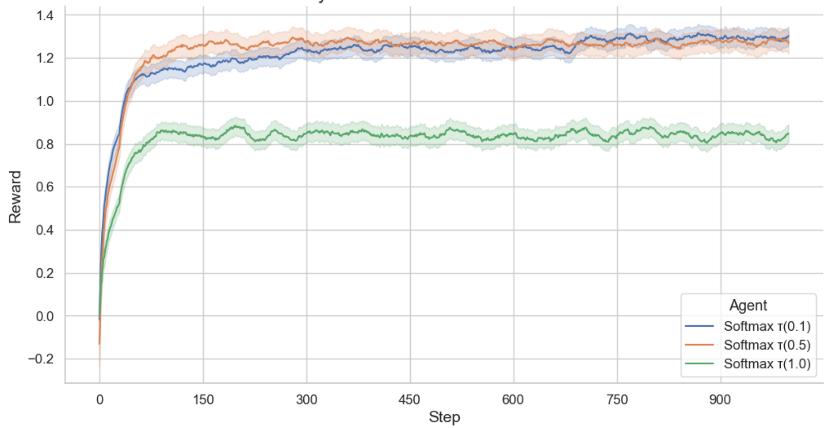
Stationary Bandit: Softmax with Different \tau Values
